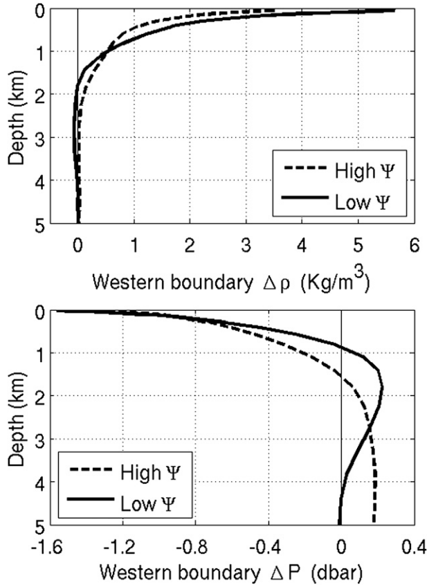
FIG. 6. Atlantic western boundary (top) meridional density difference and (bottom) pressure difference in the EOS suite. The difference is taken between 74^\circ\text{N} and the equator and shown here for the highest overturning case where \delta T = -3^\circ\text{C} (dashed lines) and for the lowest overturning case where \delta T = 9^\circ\text{C} (straight lines). The case for high overturning corresponds to a weaker meridional density difference in the western boundary, but a stronger negative pressure difference in the upper part of the ocean that changes sign at a deeper level.
