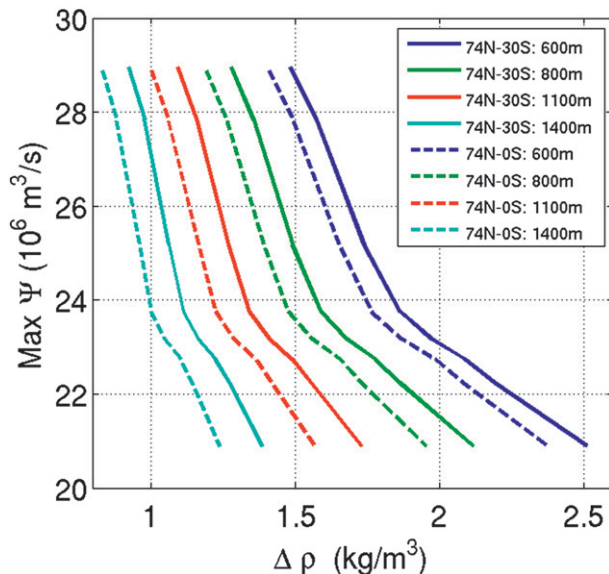
FIG. 4. The maximum overturning streamfunction \Psi in the Atlantic as a function of the meridional density difference between 74^{\circ}\text{N} and 30^{\circ}\text{S} (solid line) and the equator (dashed line) for the EOS suite. The density is vertically averaged from the surface to 600 m (dark blue), 800 m (green), 1100 m (red), and 1400 m (light blue), respectively. The inverse relationship between the AMOC and the MDD holds in all cases.
