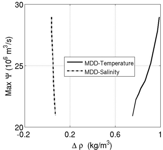
FIG. 10. The change in Atlantic maximum overturning as a function of changes in the tracer MDD (for the EOS suite). The effects of tracer temperature on the MDD (solid line) and salinity on the MDD (dashed line) are separated to distinguish them. As in previous figures, the density is vertically integrated from the surface to 1400 m and the gradient taken between the equator and 74°N. The increase in the tracer MDD with stronger AMOC found in Fig. 9 is due to an increase in the meridional temperature gradient. Changes in the salinity gradient are much smaller and of opposite sign.
