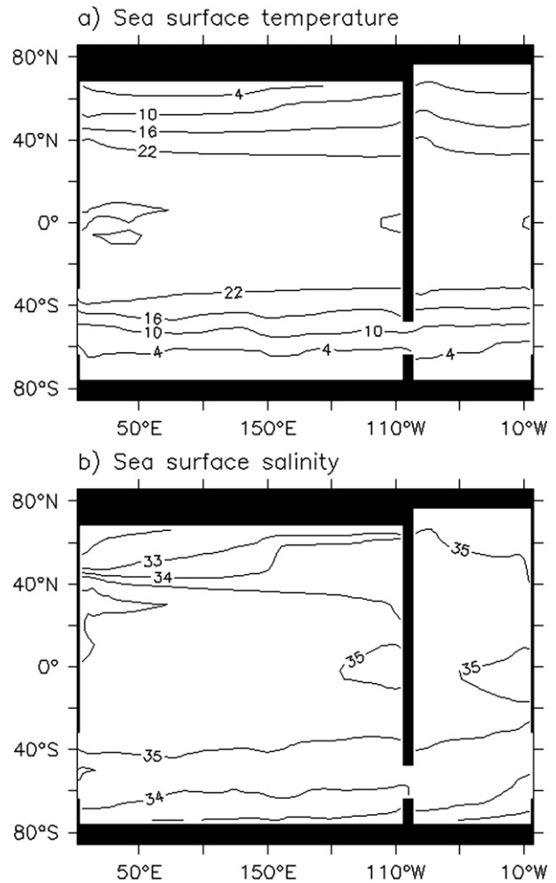
FIG. 1. Sea surface (a) temperature (°C) and (b) salinity in the control run of the EOS suite of model integrations.
